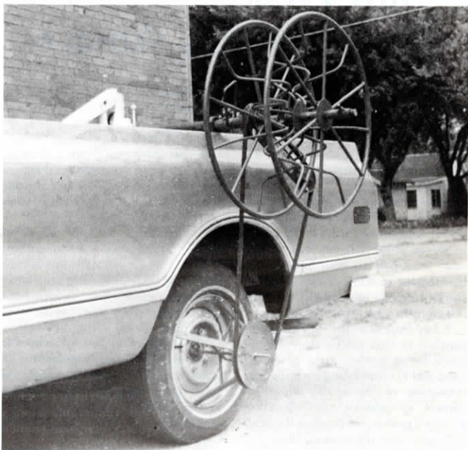
Wheel drive for the Dudley wire roller mounts on the hub without having to jack up the wheel. Spool takes up mile of smooth wire, 100 rods of barbed wire.
