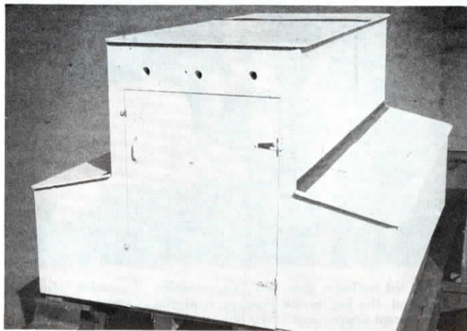
Inside dimensions of the climate controlled Little Sambo farrowing hut are 5 ft. wide, 6.5 ft. long and 4 ft. high. Side doors lift up for easy access to small pigs.
