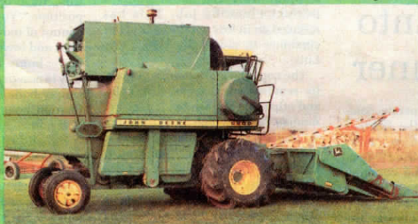
Dryer mounts above grain tank to minimize modification.
