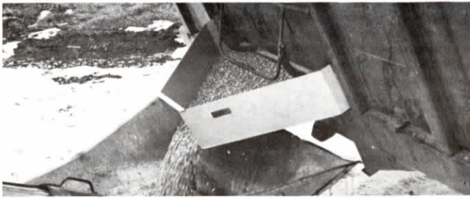
One grain-saving chute can be used interchangeably on several trucks or wagons.
