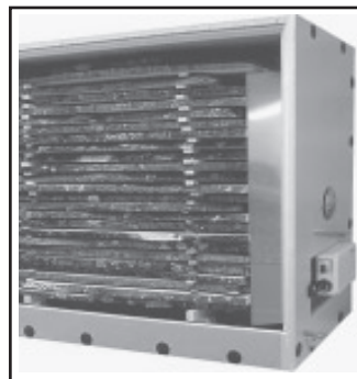
Temporary kilns are made of sheets of 2-in. Styrofoam, held together with clips and screws supplied with the kit. Can be used to dry sawn lumber or firewood.
