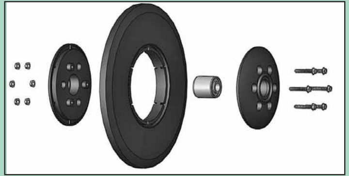
Wheels come in 10 or 12-in. dia., fitted with a 5/8-in. bearing.
