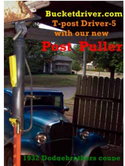
New post puller attachment consists of a pin that locks onto fence post notch so that posts can be pulled quickly with driver.
