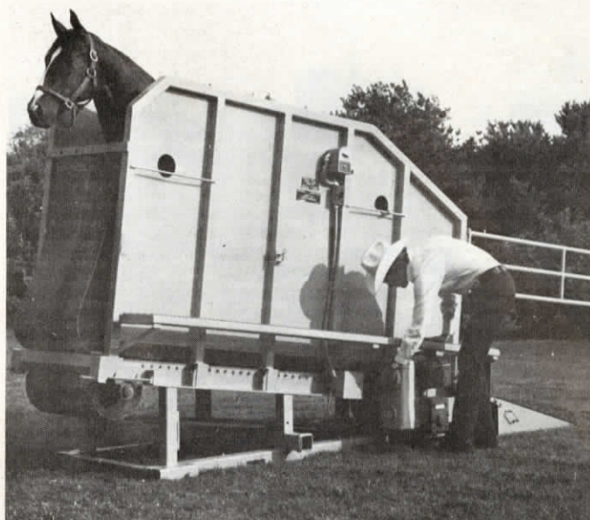
Treadmill platform is equipped with 40 rollers with sealed ball bearings. Measures 4 ft. (for cattle or horses) or 3 ft. (for horses only) wide, 10 ft. long and 7 ft. high.
