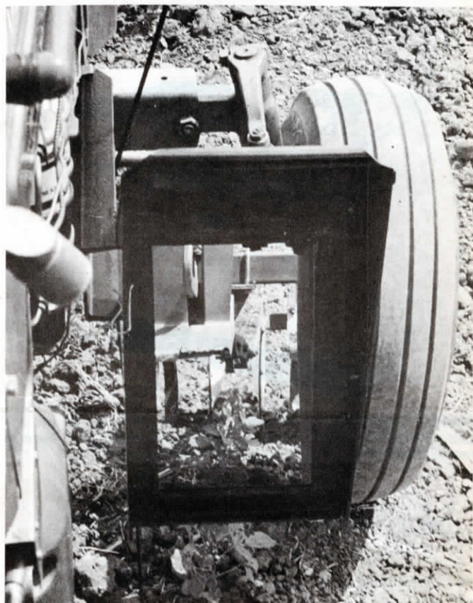
Culti-vision comes with row guide rod and protective cover which is closed to protect mirror when traveling on gravel roads.
