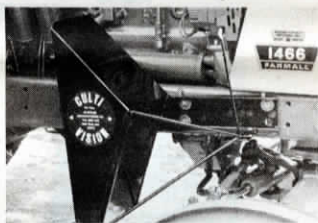
Standard model mounts on right side as viewed from driver's seat. Units built in reverse for left side also available.
