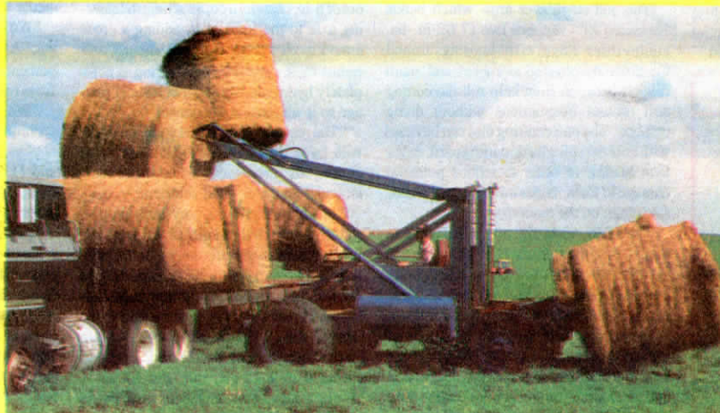
Round Bale Handler - Self-propelled bale hauler can handle four bales at a time, each mounted on independently controlled bale spears that tip up and down. Operator platform swivels 180° to make loading rear-mounted bales easy.
