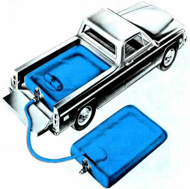
Popular 500-gal. Flexitank for pickups measures 60 in. by 96 by 20 in. Drawings show how tanks can be placed in buildings, above ground or underground.
