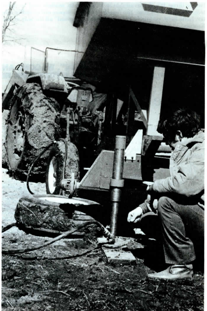
Axle cap helps prevent jack from slipping out from under an axle. Hydraulically-operated jack operates off any tractor or other system with 3000 psi or less.
