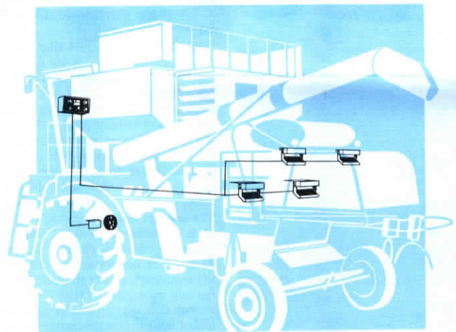
Sensors linked to control console in cab monitor grain loss at straw walker and shoes, and ground speed.
