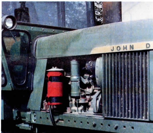
Phoenix electric oil refiner, designed for do-it-yourself installation, is equipped with a heating element to remove moisture from oil as it refines it.
