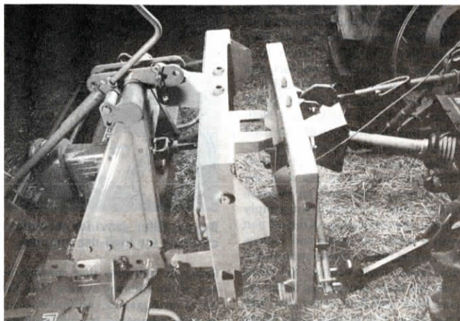
Special 3-pt. pto frame locks into implement-mounted frame.
